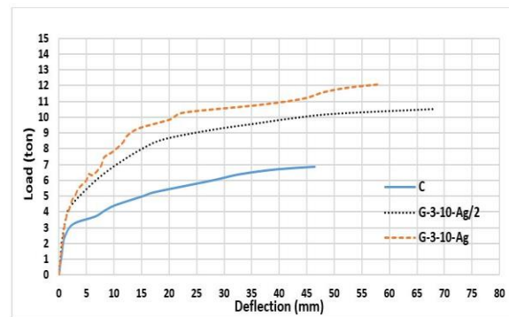
Fig.14: Comparison between Load-Central deflection relationships of the specimens (G-3-10-Ag/2), (G-3-10-Ag), and (C).
