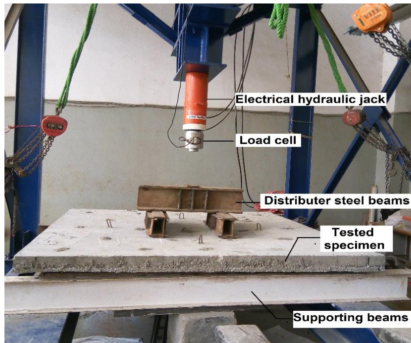
Fig.5: The test set-up.
