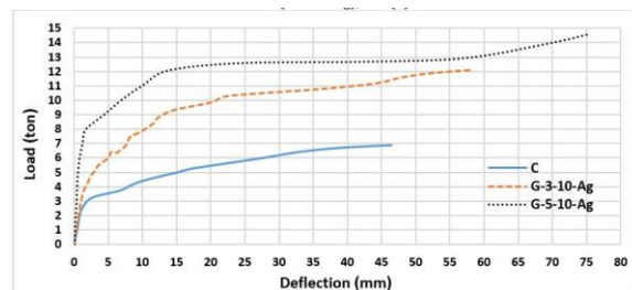
Fig.9: Comparison between Load-Central deflection relationships of the specimens (G-3-10-Ag), (G-5-10-Ag), and (C).
