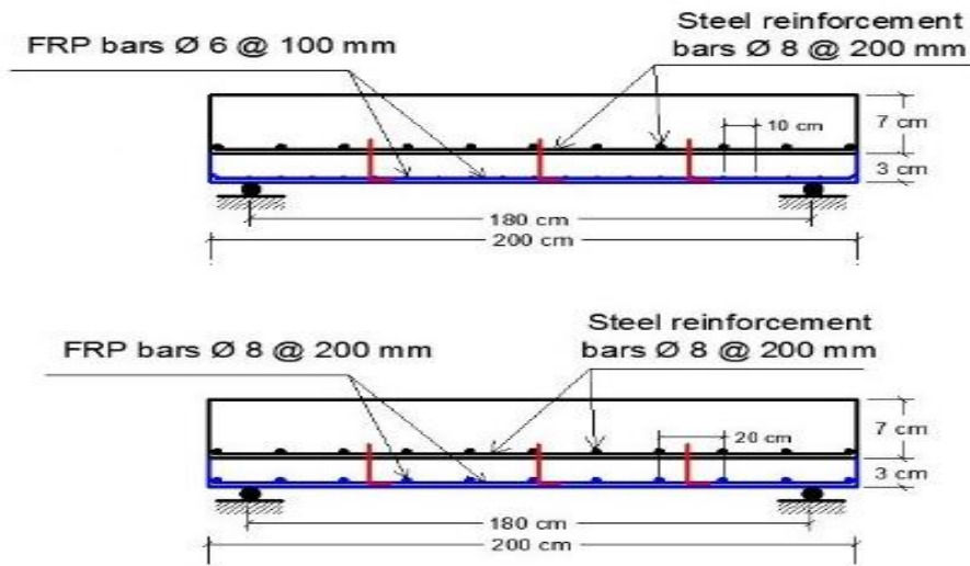
Fig. 3: Adding lower concrete layer reinforced by FRP bars.
