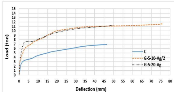
Fig.12: Comparison between Load-Central deflection relationships of the specimens (G-5-10-Ag/2), (G-5-20-Ag), and (C).
