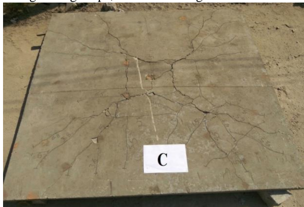
Fig.18: Cracking pattern of specimen(C).
