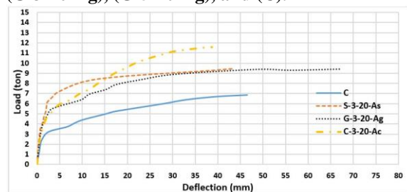
Fig.10: Comparison between Load-Central deflection relationships of the specimens (S-3-20-As), (G-3-20-Ag), (C-3-20-Ac), and (C).
