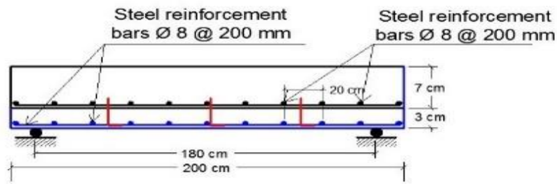
Fig.2: Adding lower concrete layer reinforced by steel reinforcement mesh.
