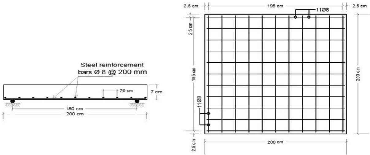
Fig.1: Dimensions and reinforcement details of the control specimen and the other specimens. prior to strengthening
