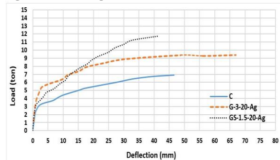
Fig.16: Comparison between Load-Central deflection relationships of the specimens (G-3-20-Ag), (GS-1.5-20-Ag), and (C).
