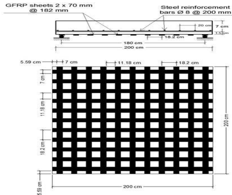
Fig. 4: Adding lower concrete layer reinforced externally by bonded GFRP strips.
