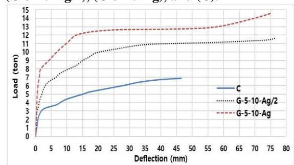
Fig.15: Comparison between Load-Central deflection relationships of the specimens (G-5-10-Ag/2), (G-5-10-Ag), and (C).
