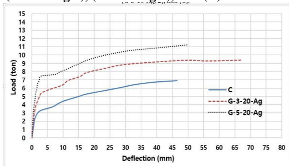
Fig.8: Comparison between Load-Central deflection relationships of the specimens (G-3-20-Ag), (G-5-20-Ag), and (C).
