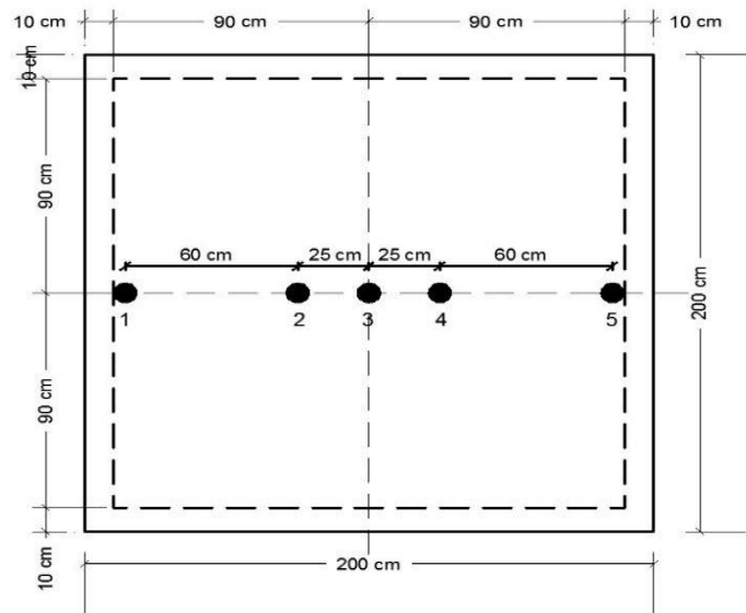
Fig.6: LVDT locations (bottom side).
