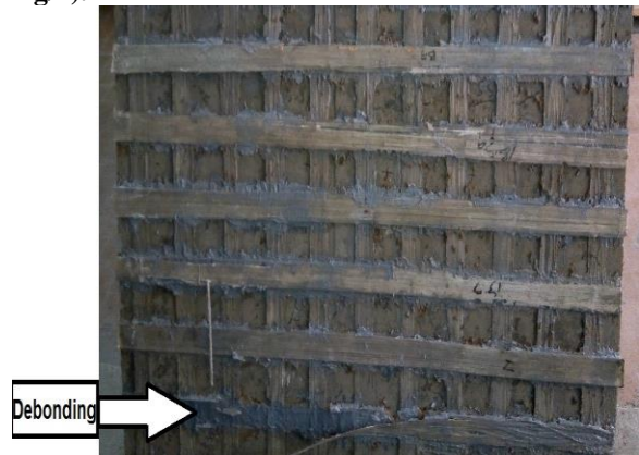
Fig.20: Deponding shape for specimen (GS-1.5-20-Ag).
