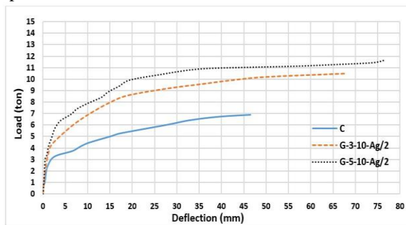
Fig.7: Comparison between Load-Central deflection relationships of the specimens (G-3-10-Ag/2), (G-5-10-Ag/2), and (C).
