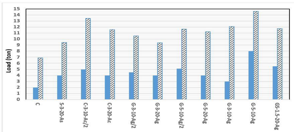
Fig.17: Cracking and ultimate load for all test specimens
