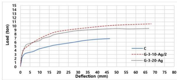
Fig.11: Comparison between Load-Central deflection relationships of the specimens (G-3-10-Ag/2), (G-3-20-Ag), and (C).
