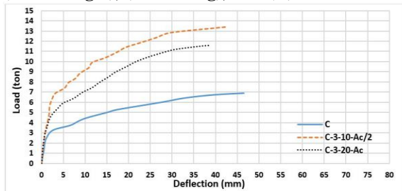
Fig.13: Comparison between Load-Central deflection relationships of the specimens (C-3-10-Ac/2), (C-3-20-Ac), and (C).
